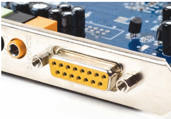
• Figure 3.23 Legacy joystick/MIDI port
