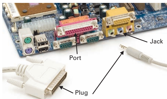
• Figure 3.8 Plug, port, and jack
