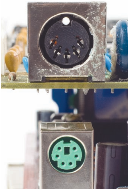
• Figure 3.9 DIN (top) and mini-DIN (bottom) connectors
