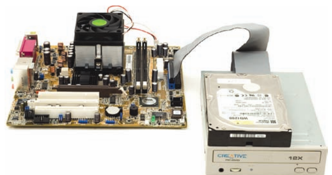
• Figure 3.44 Hard drive and DVD drive
