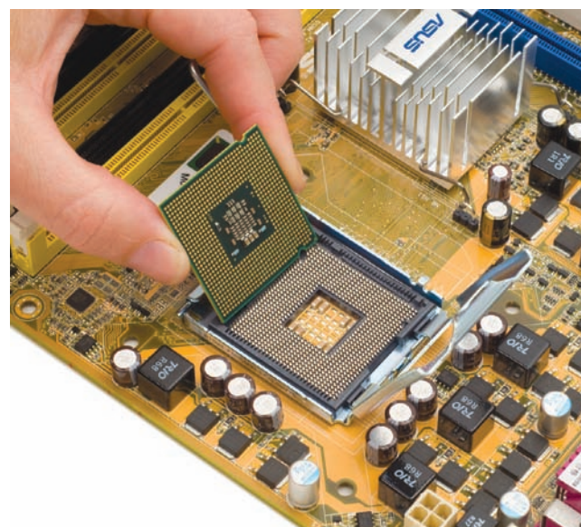
• Figure 3.37 CPU and matching socket
