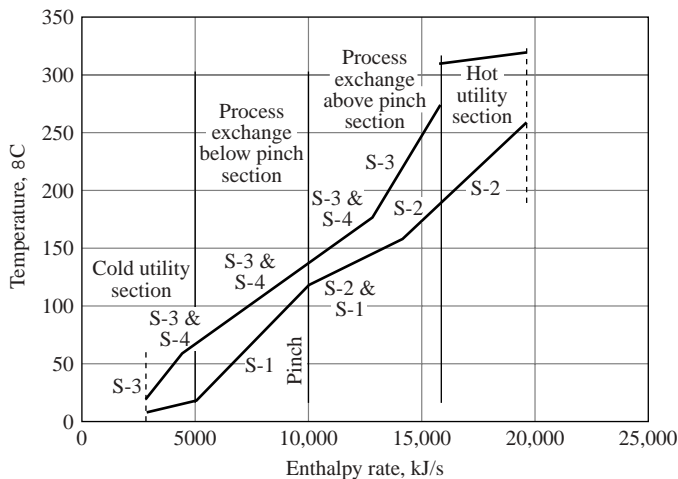
Figure 9-18 Balanced composite diagram with 20^\circ\text{C} approach temperature
