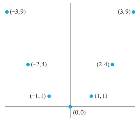
FIGURE 9 The Graph of f(x) = x^2 from \mathbb{Z} to \mathbb{Z} .
